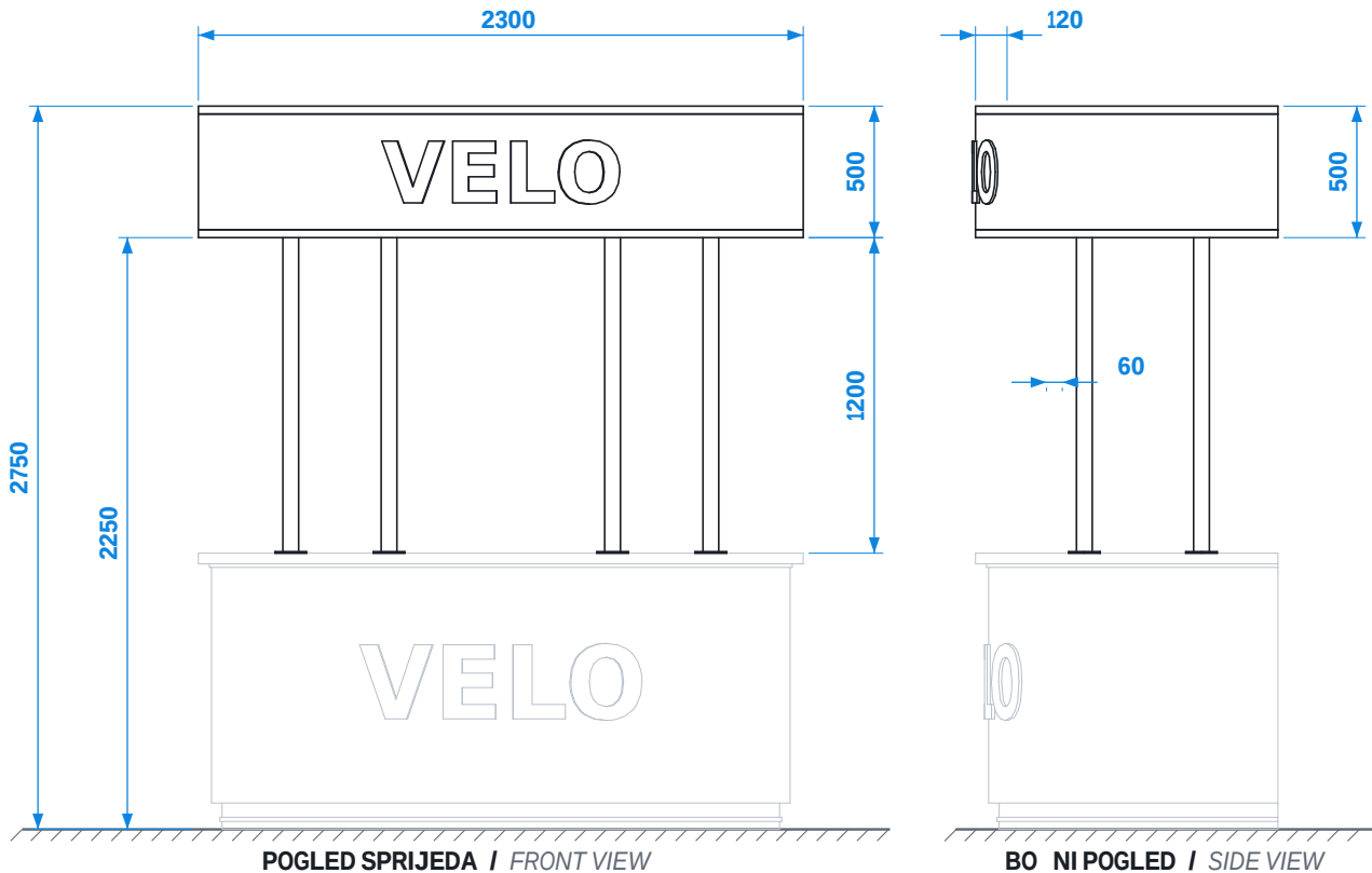
2D POGLED S MJERAMA / 2D view with dimensions
