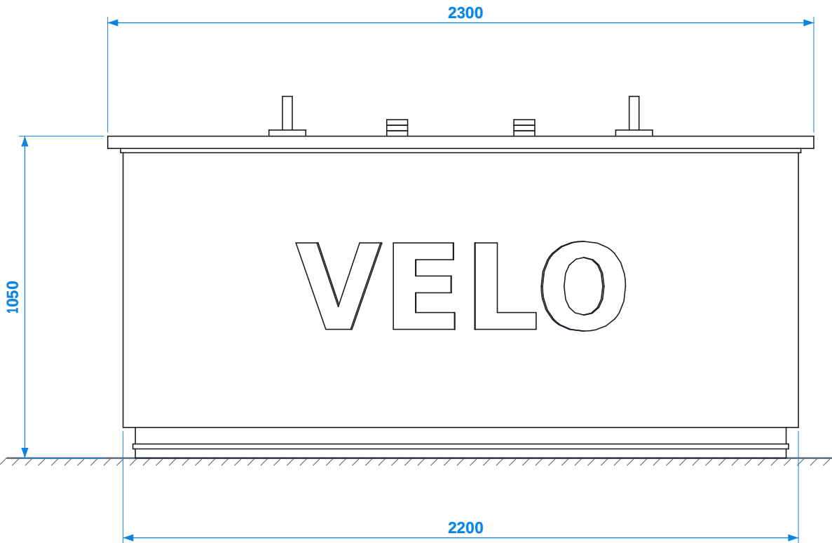
POGLED SPRIJEDA / FRONT VIEW
