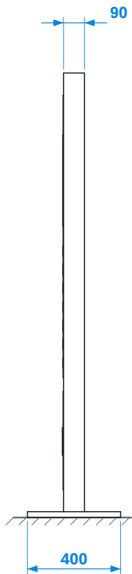
BO NI POGLED / SIDE VIEW
