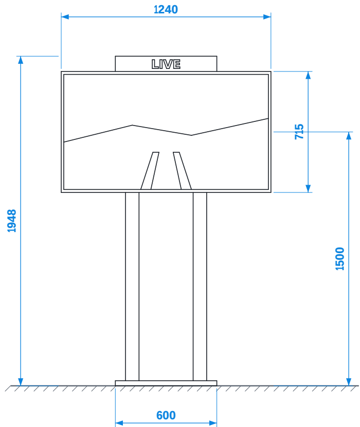
POGLED SPRIJEDA / FRONT VIEW
