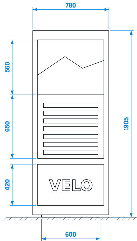
POGLED SPRIJEDA / FRONT VIEW
