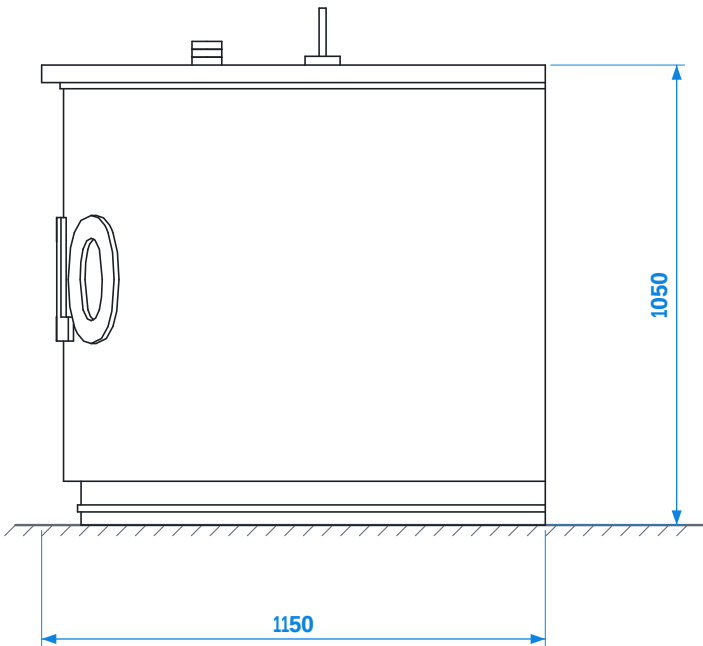
BO NI POGLED / SIDE VIEW
