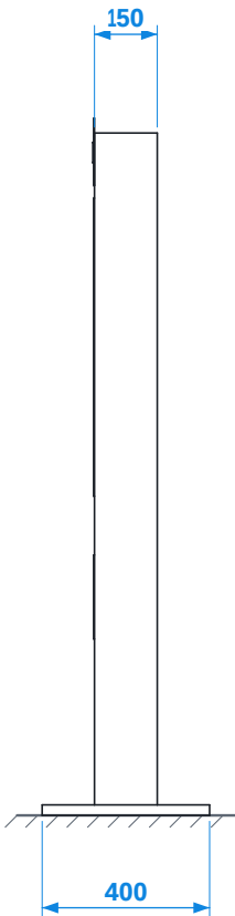
BO NI POGLED / SIDE VIEW
