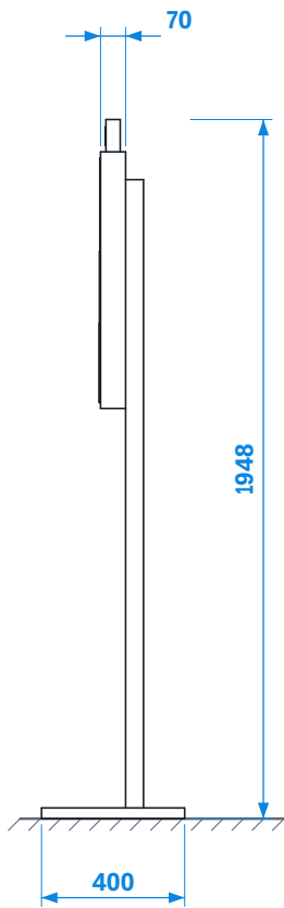
BO NI POGLED / SIDE VIEW
