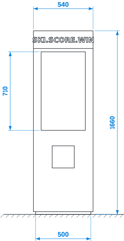
POGLED SPRIJEDA / FRONT VIEW
