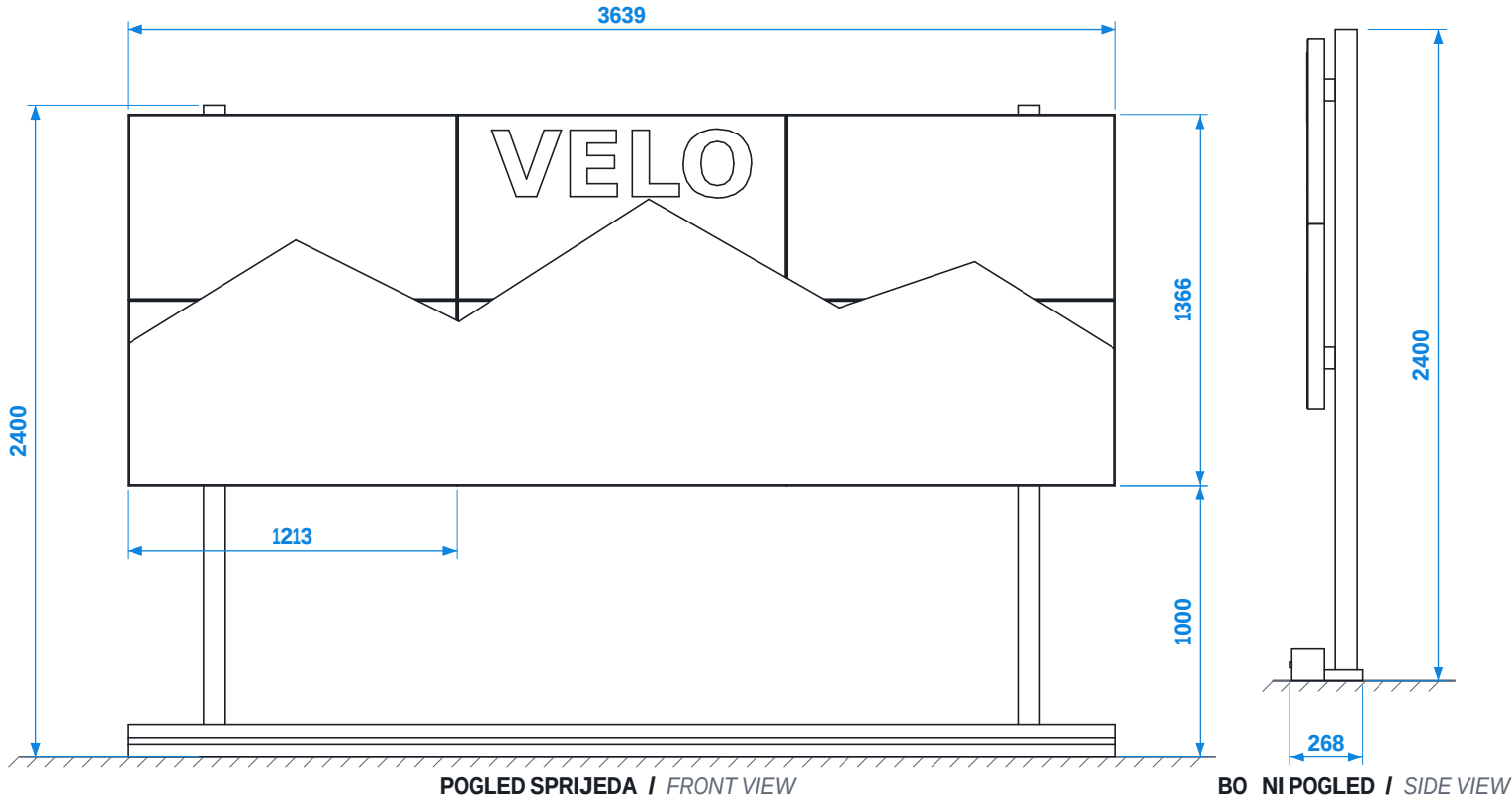
2D POGLED S MJERAMA / 2D view with dimensions
